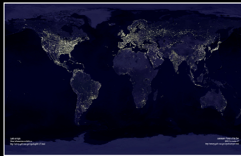
Images © NOAO Globe At Night
